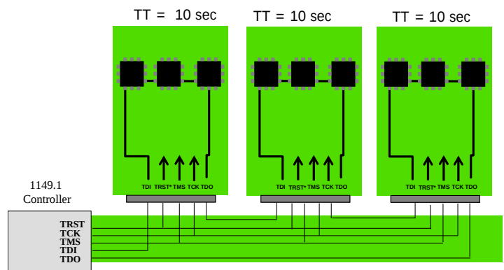
Figure 1. Daisy Chained PCBs - No Test Time Reduction
