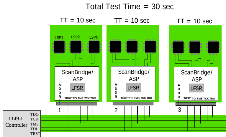
Figure 2. Multi-drop Test – No Test Time Reduction
