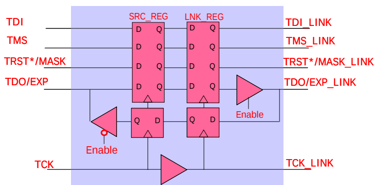
Figure 9. PTB Synchronizer Details
